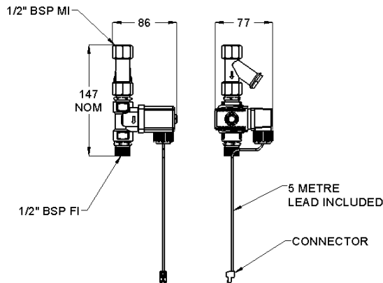
52056 - SOLENOID ASSEMBLY
